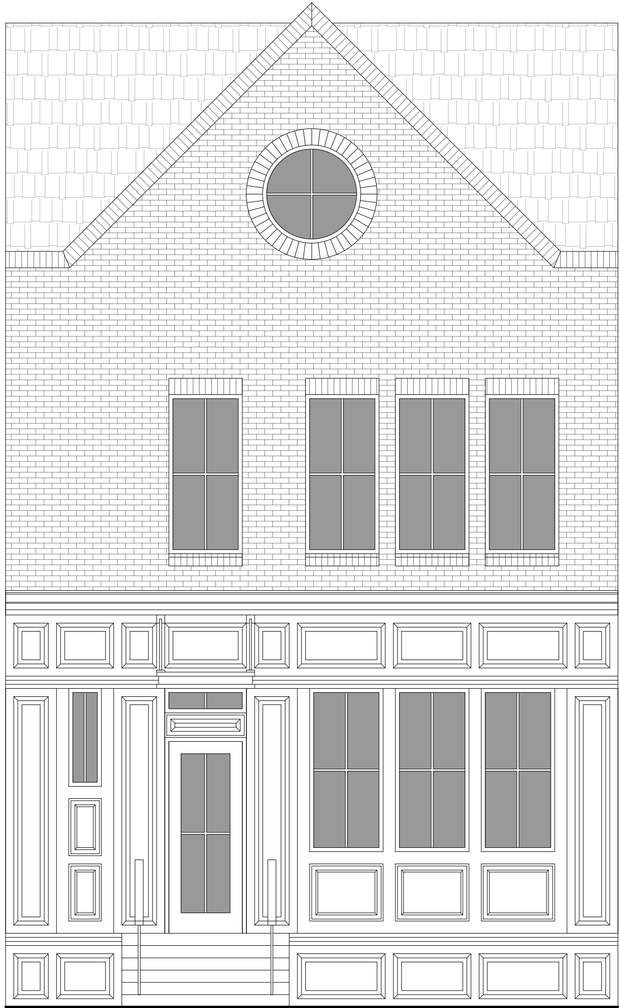
FRONT ELEVATION
