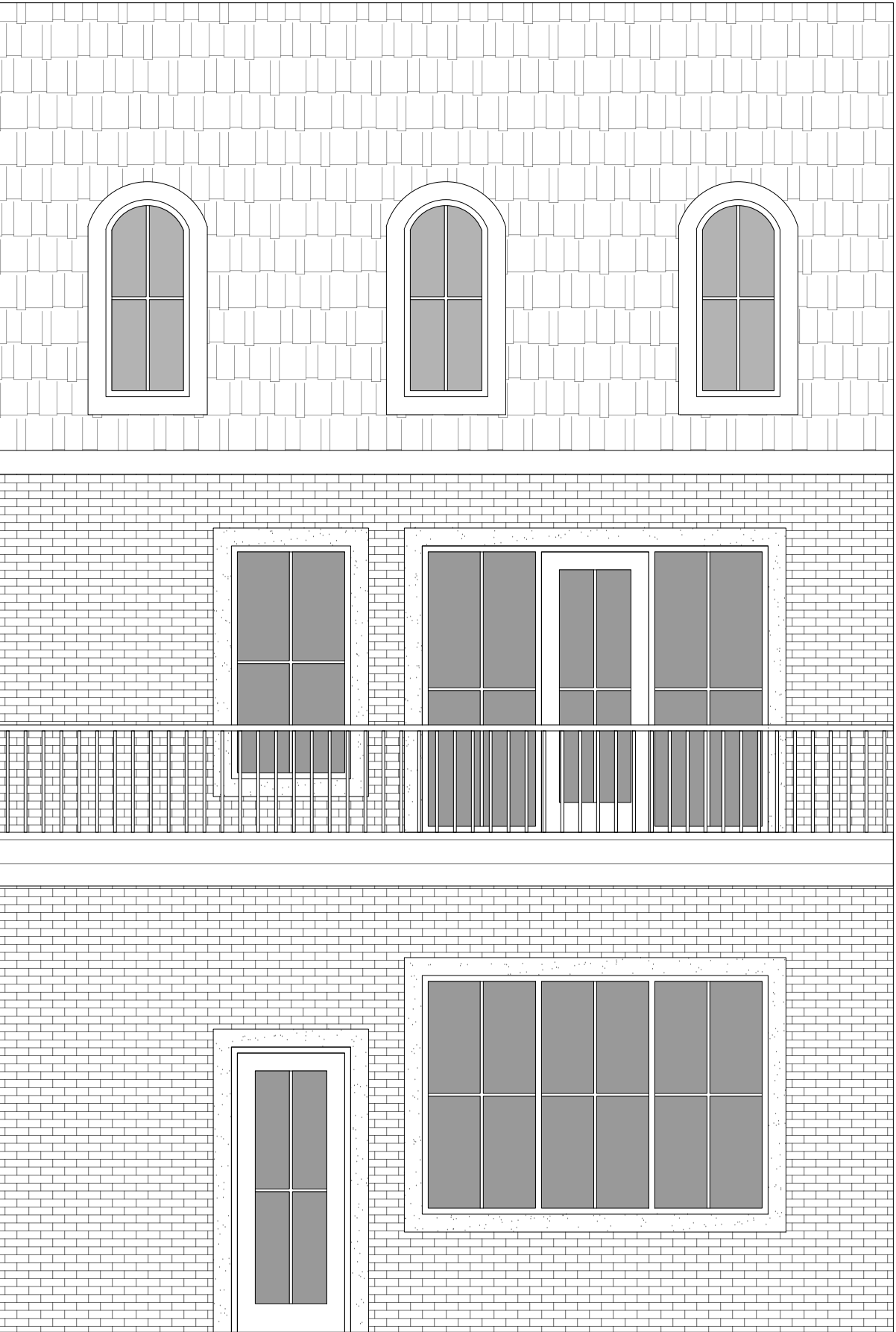
REAR ELEVATION
