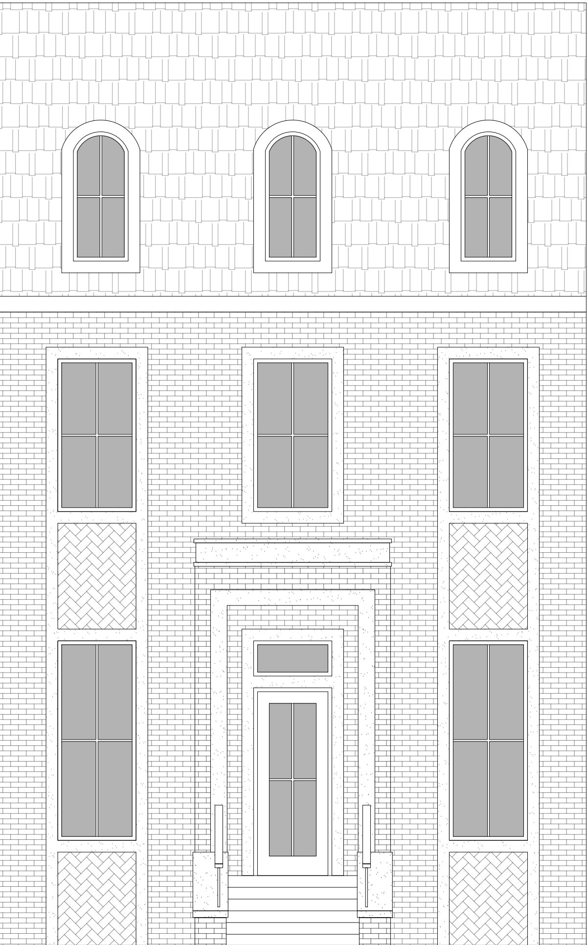
FRONT ELEVATION
