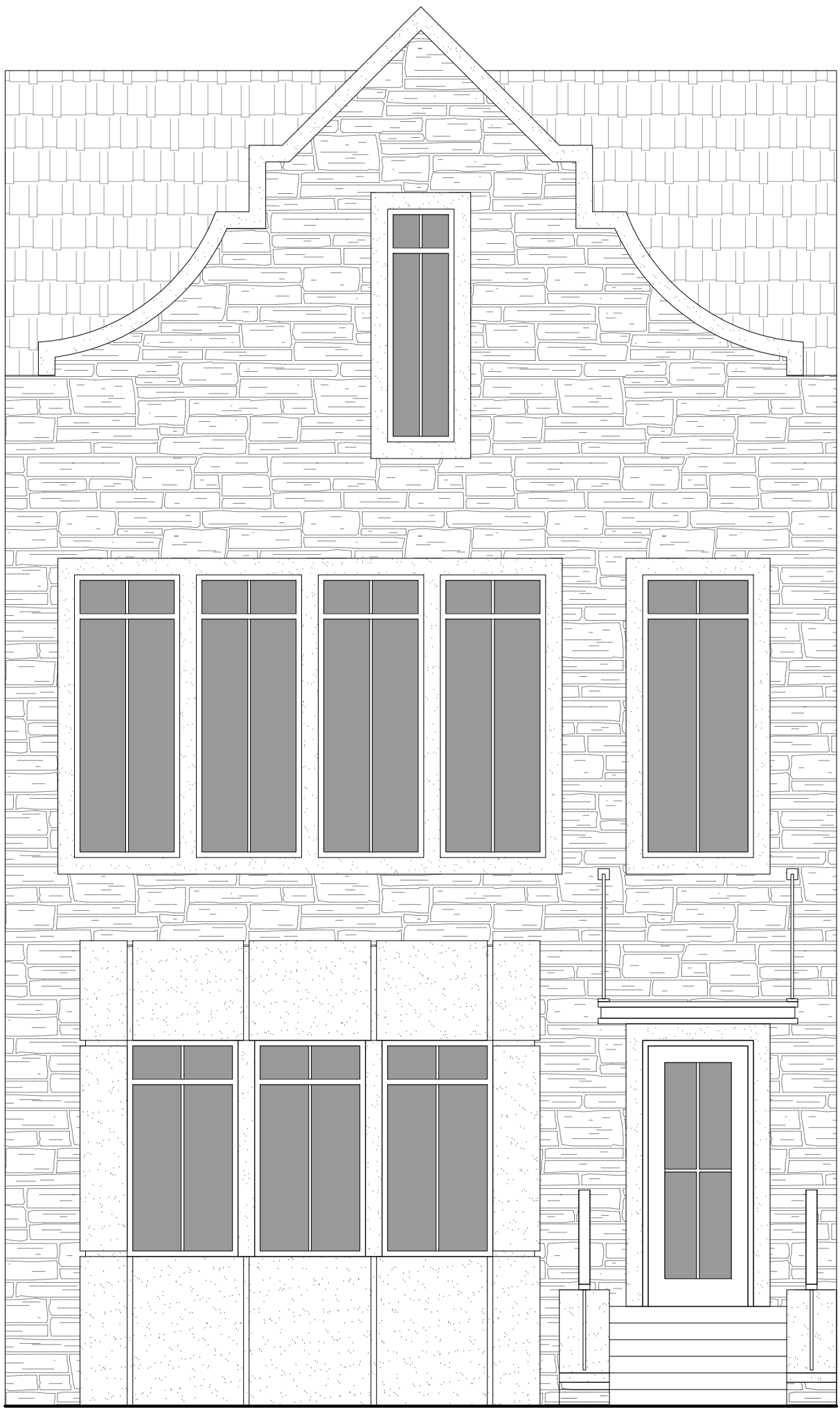
FRONT ELEVATION
