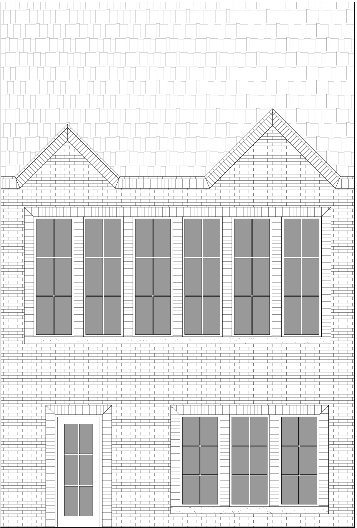
REAR ELEVATION
